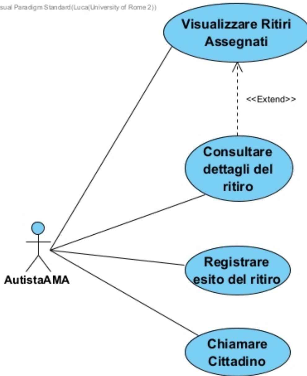
Figura 3: Use Case Diagram — Autista AMA
